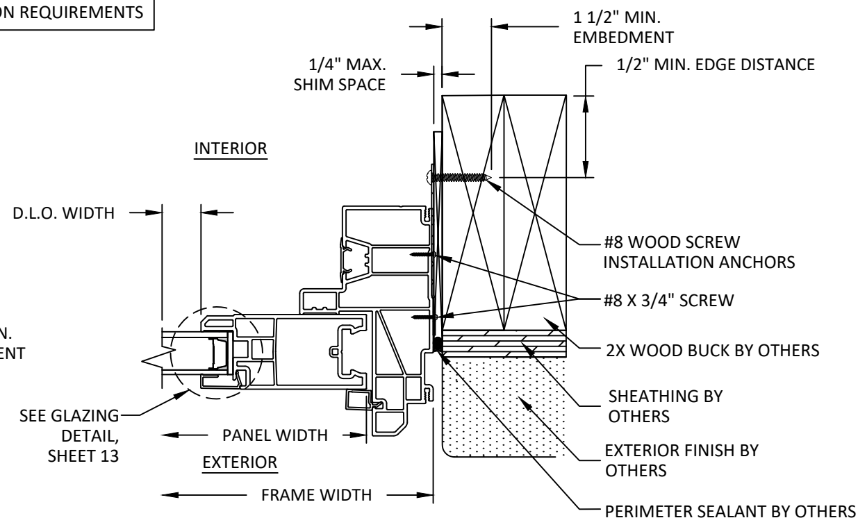
D 11 HORIZONTAL SECTION CLIP INSTALLATION WOOD SUBSTRATE
