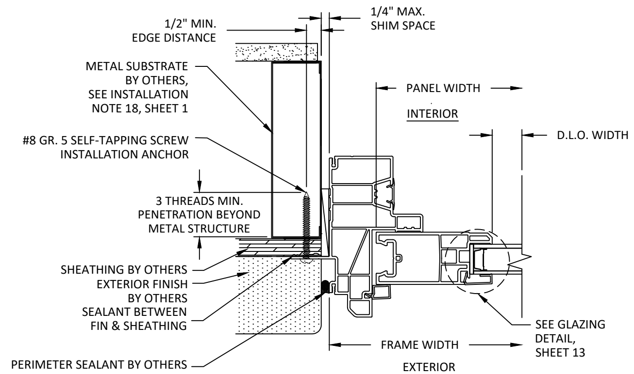
B 9 HORIZONTAL SECTION NAIL FIN INSTALLATION METAL SUBSTRATE
