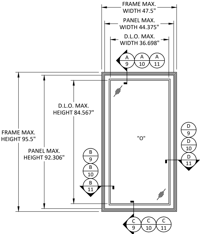
TYPICAL ELEVATION
