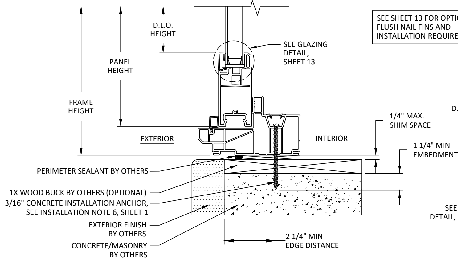
C 10 VERTICAL SECTION THROUGH FRAME INSTALLATION CONCRETE/CMU SUBSTRATE
